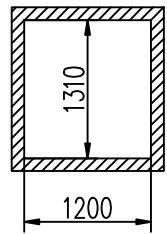
Shaft plan view
