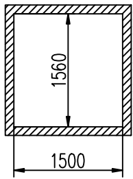
Shaft plan view
